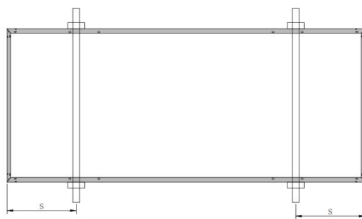
#4 长框夹块
